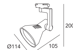
T-106/xx-PAR30
