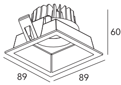
R-SQ-201/xx-COB-7W-3K
