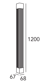
VA-303 LED 1X18W Stainless Steel Polished + Opal glass
